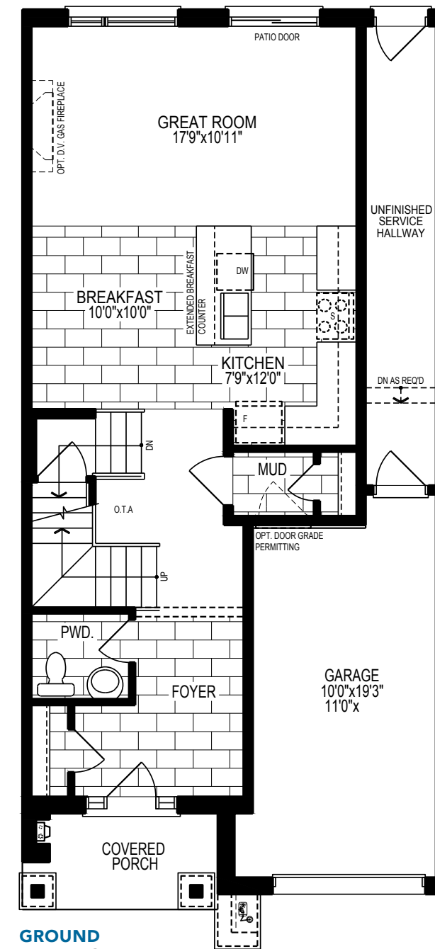
GROUND ELEVATION A INTERIOR UNIT
