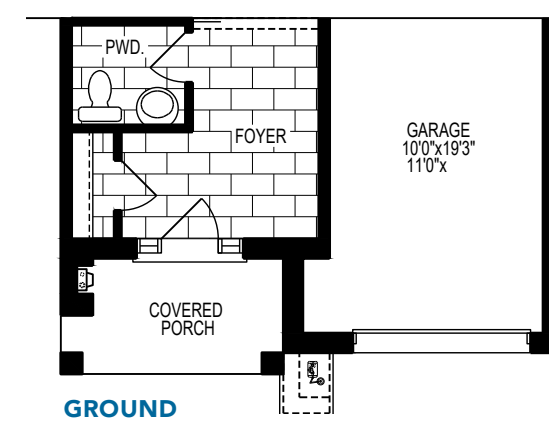
GROUND ELEVATION B INTERIOR UNIT
